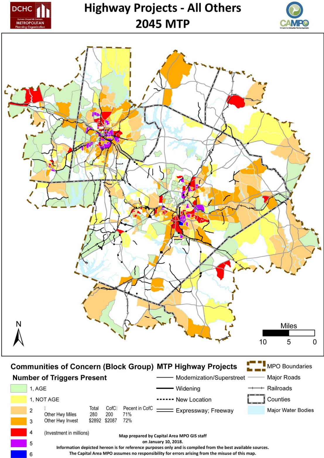
Figure 9.2.5 Title VI Compliance: CAMPO/DCHC All Other Roadway
