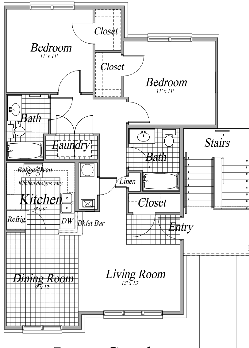
Long Creek 2 Bedroom Plan - 1,001 SF
